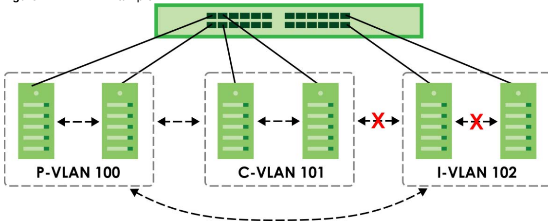
Figure 11 PVLAN Example 1
