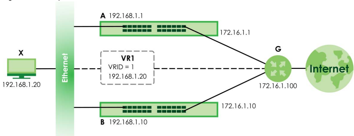
Figure 15 Example: VRRP
