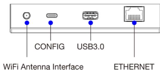
▲ Description of Internal NovaStar T10 Controller' s External Interfaces
